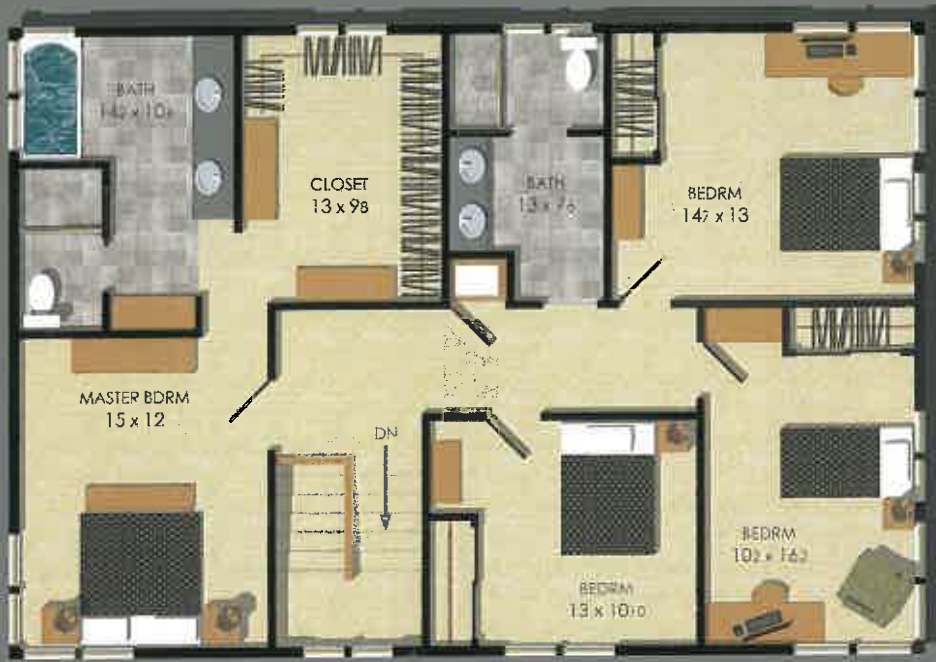
2 ND FLOOR 1,350 SF
